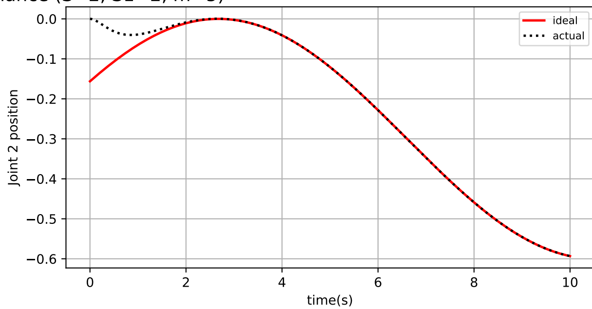
Position Tracking Performance (S=2, S1=2, m=5)
